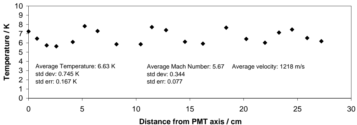
6.6K H 2 Nozzle Q H 2 = 32.2 set, P chamber = 0.088 mbar, P resevoir = 31.1 mbar
